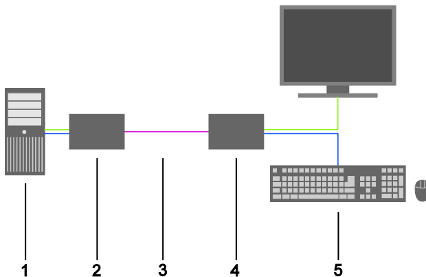
KVM-Extender (Single-Head)
